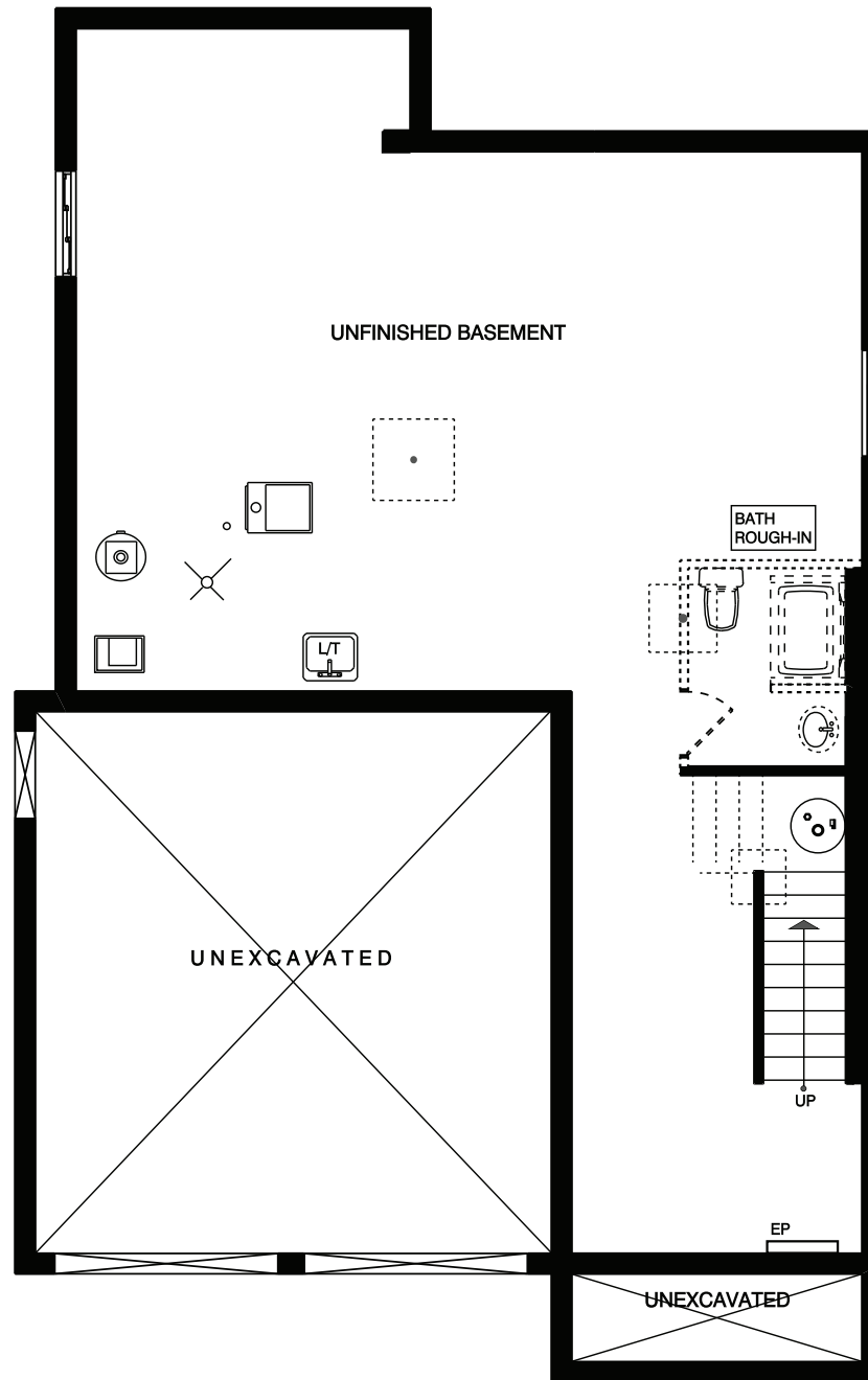
FOUNDATION LAYOUT (unfinished)
