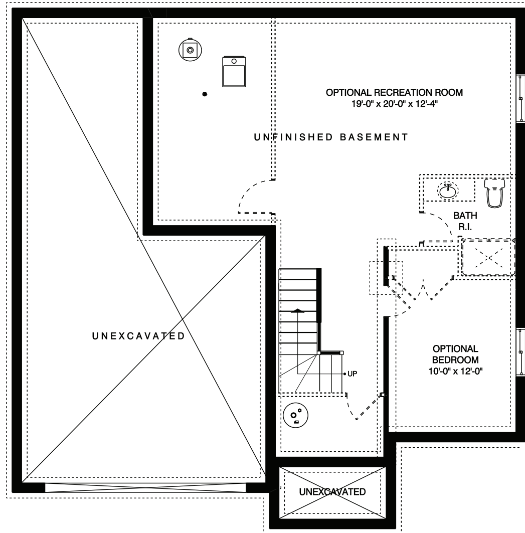
FOUNDATION LAYOUT 624 SQ. FT. OPTIONAL FINISHED AREA
