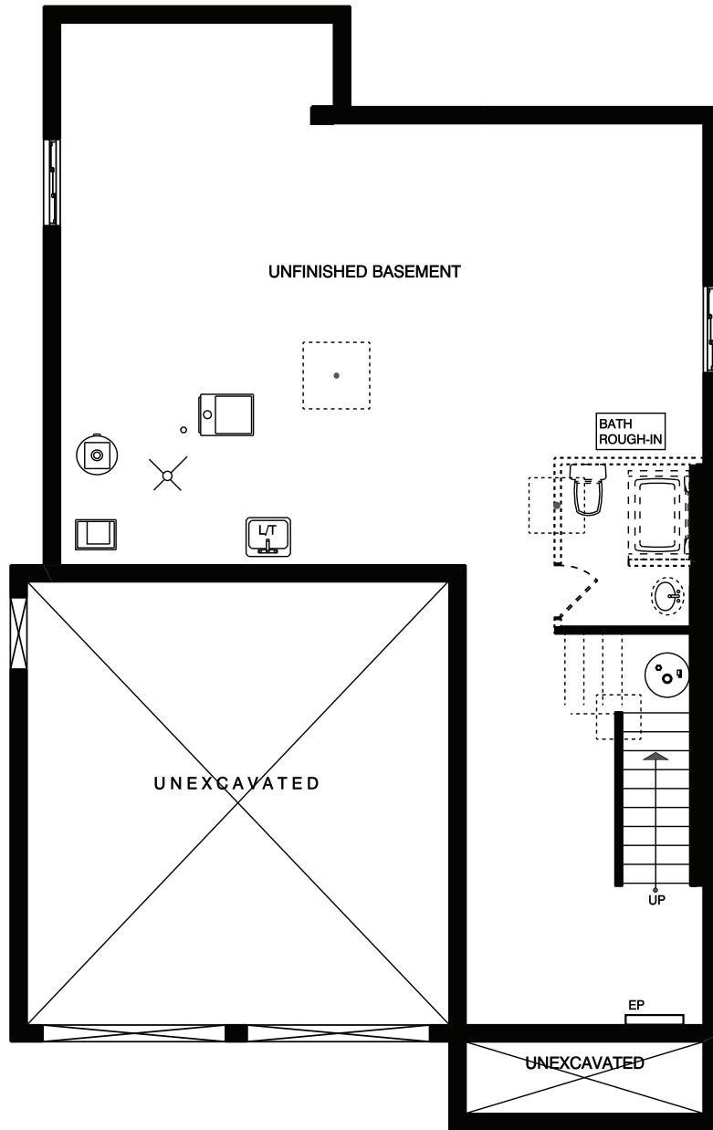
FOUNDATION LAYOUT (unfinished)
