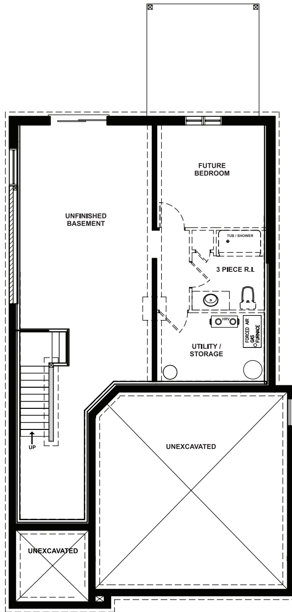
FOUNDATION LAYOUT (unfinished)
