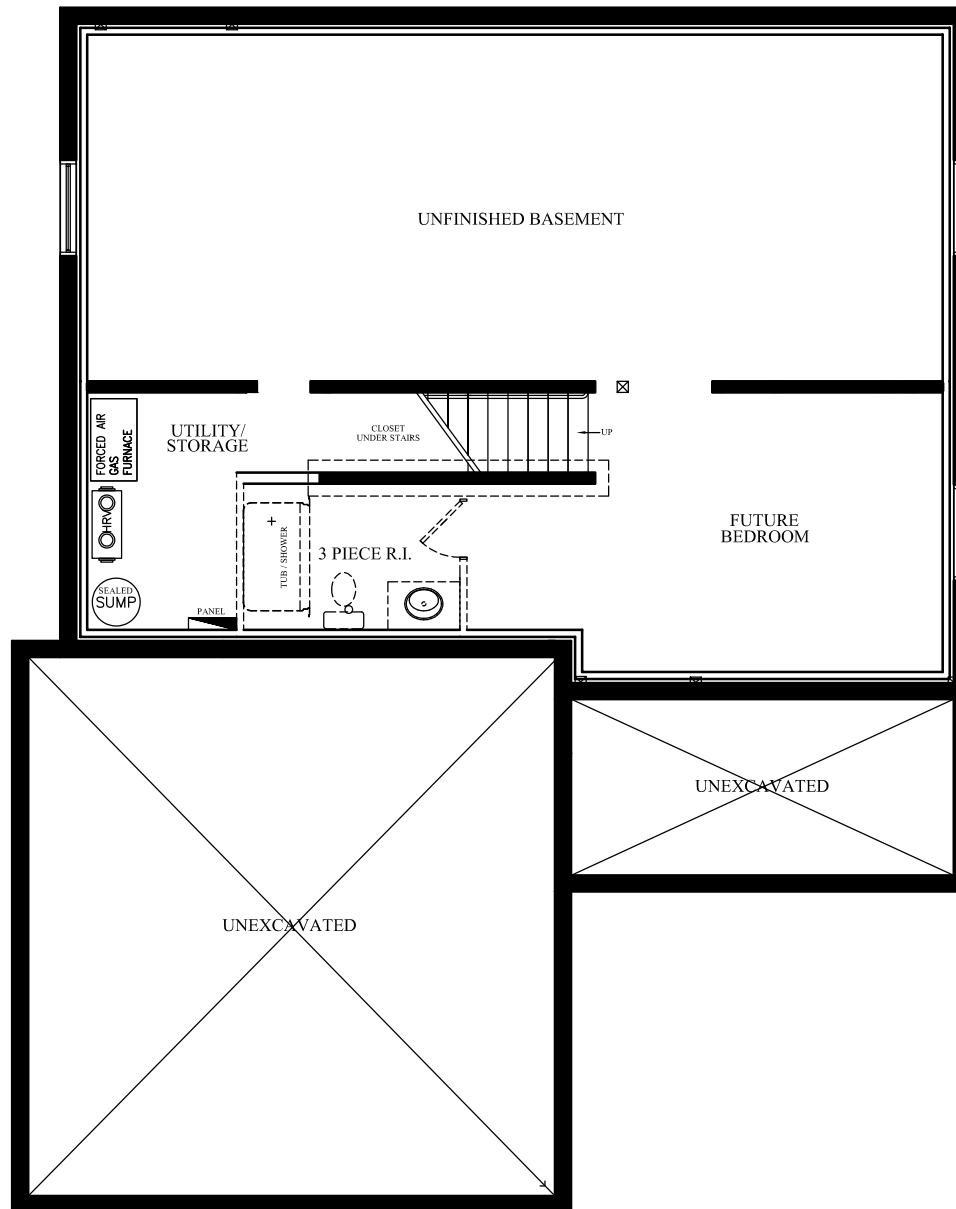
FOUNDATION LAYOUT
