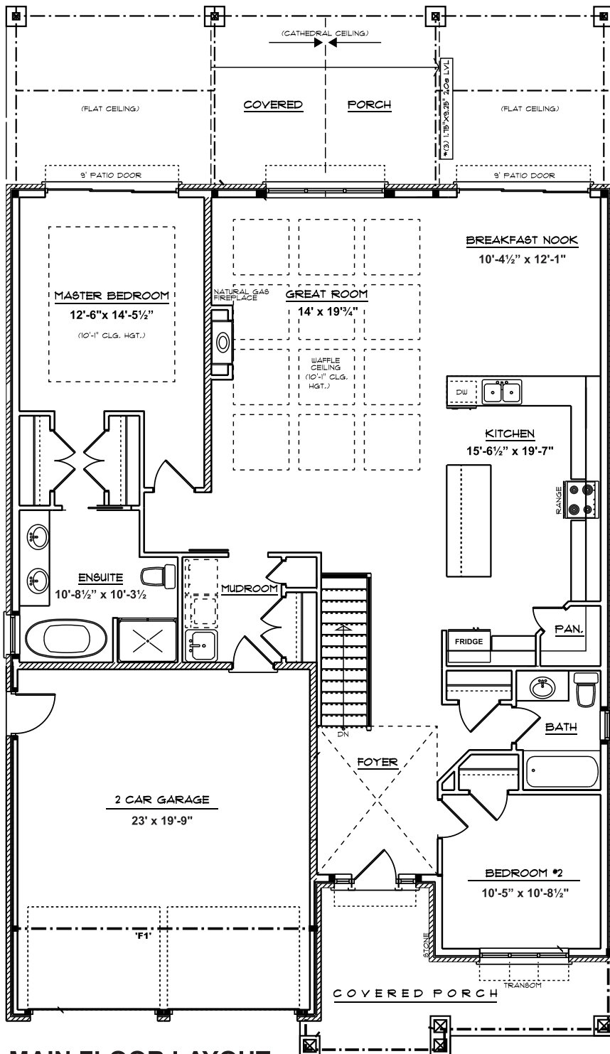
MAIN FLOOR LAYOUT 1705 SQ. FT.
