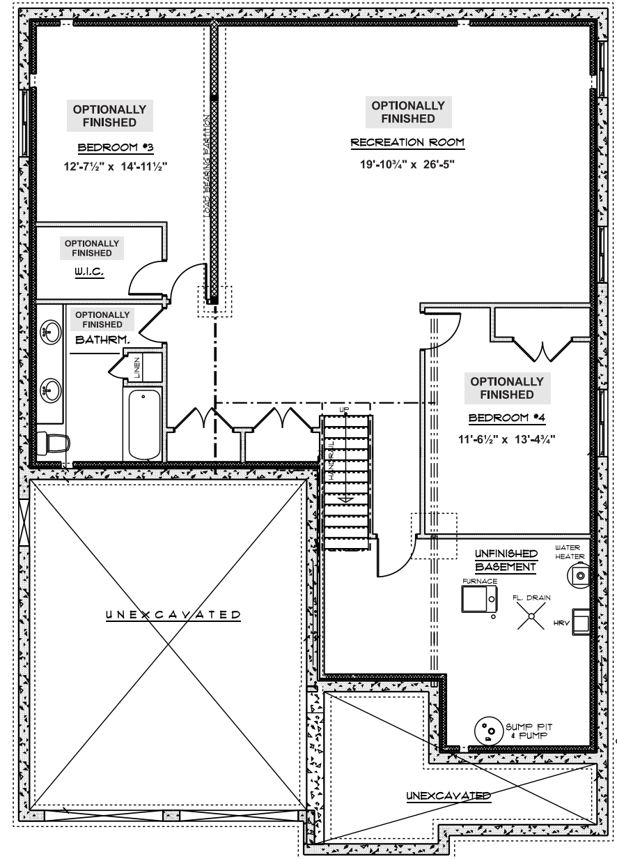
BASEMENT LAYOUT 1296 SQ. FT. (OPTIONALLY FINISHED AREA)
