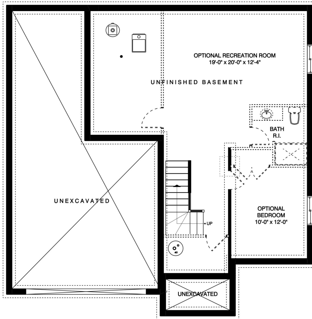
FOUNDATION LAYOUT 624 SQ. FT. OPTIONAL FINISHED AREA
